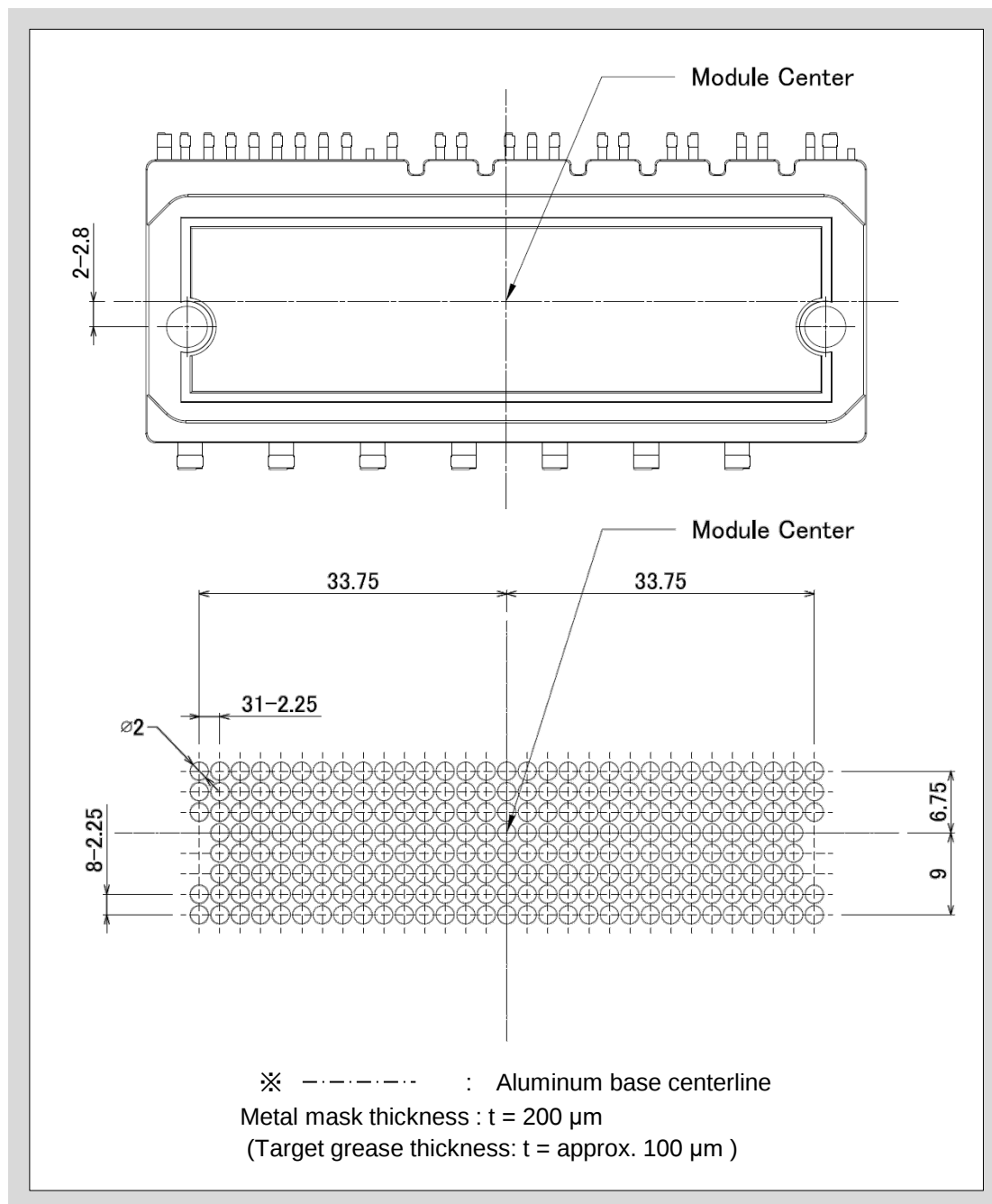
Fig. 8-1 Stencil mask drawing for thermal grease application (recommended)
