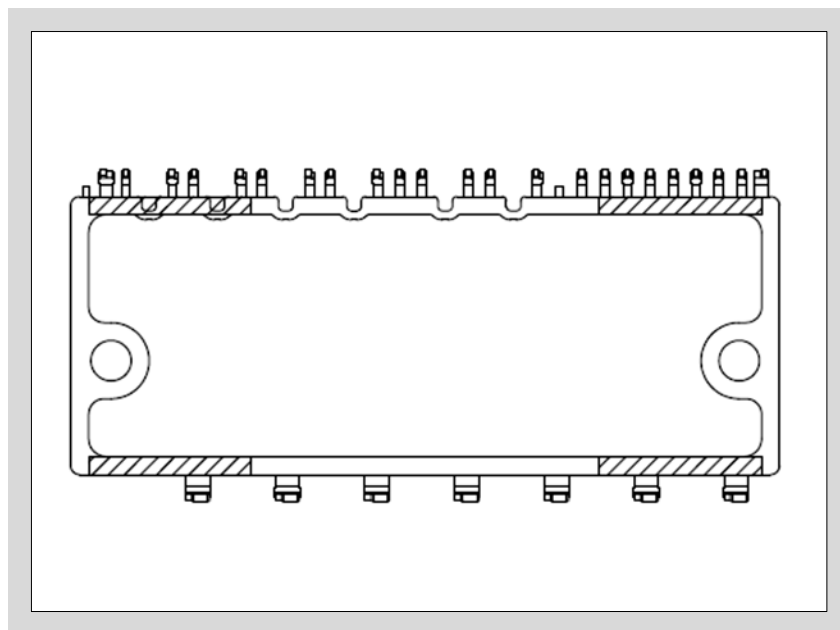
Fig. 4-1 Spacer installation position
