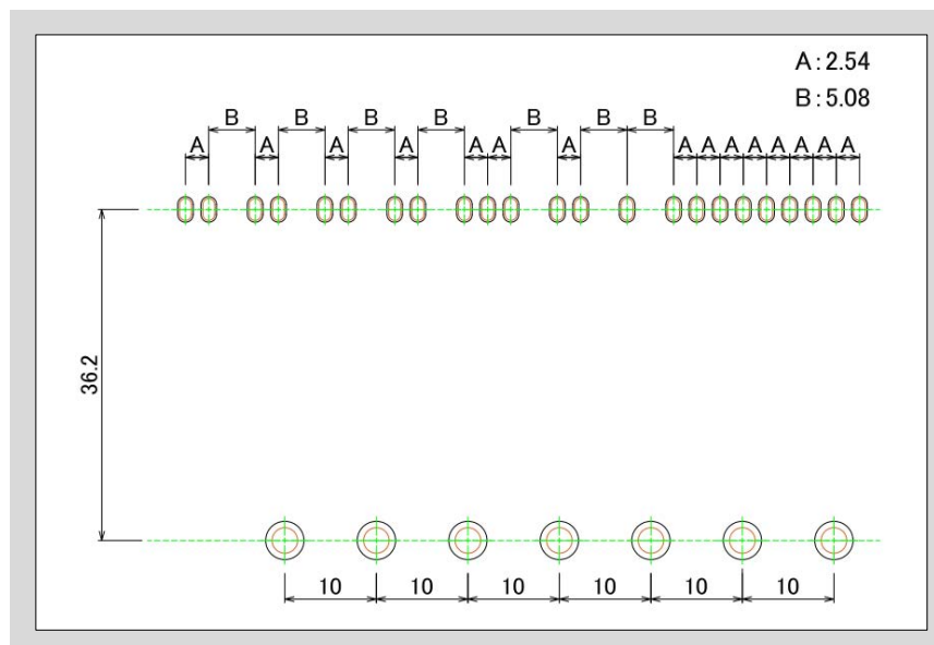
Fig. 3-3 Through hole layout
