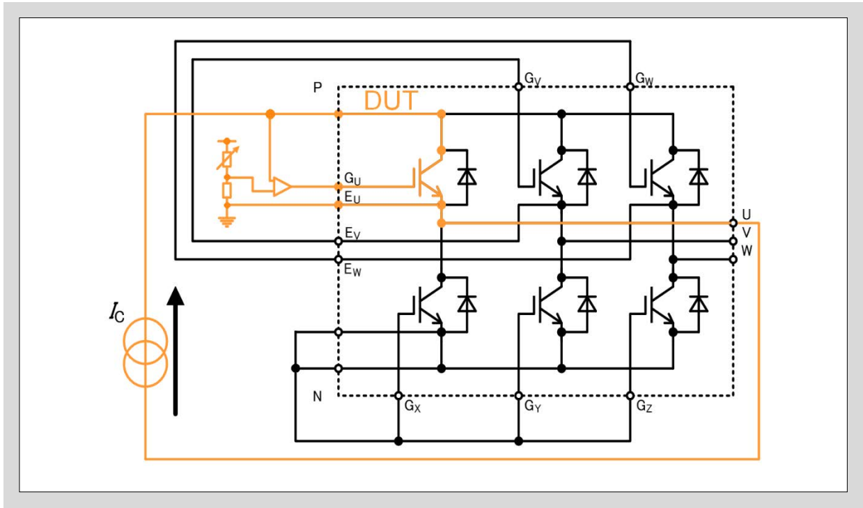
Fig.1 Equivalent test circuit
