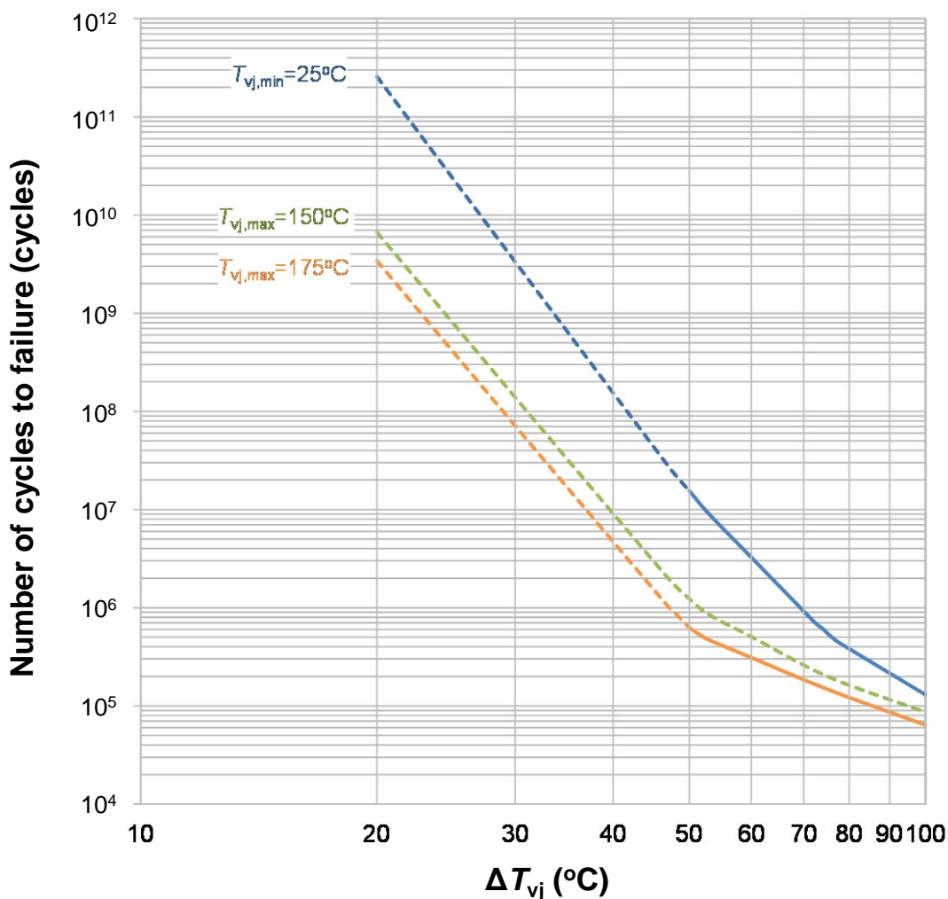
Fig.4 \Delta T_{vj} power cycling capability curve
