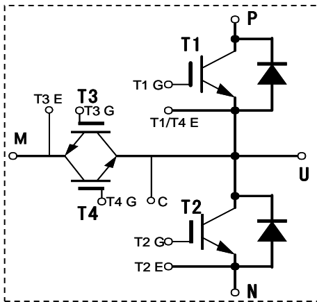
Equivalent circuit
