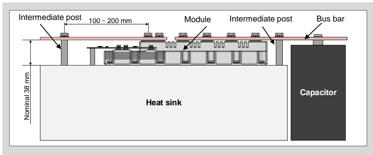
Fig.5 Example of connecting to bus bar without applying stress to the terminals (M272)
