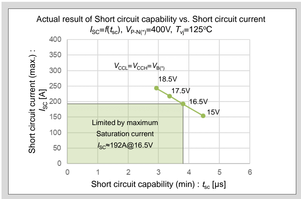
Fig.4 6MBP30XSJ(K)065-50 Short circuit capability and SCSOA
