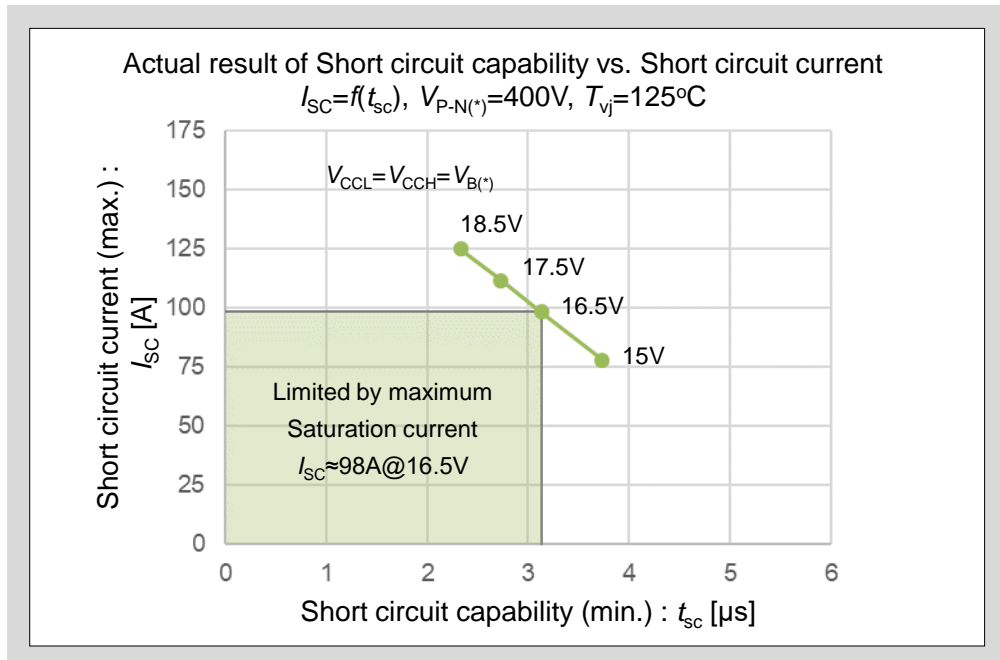
Fig.2 6MBP15XSJ(K)065-50 Short circuit capability and SCSOA
