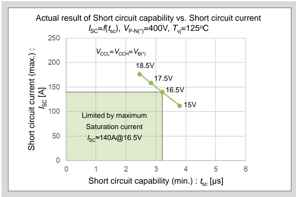
Fig.3 6MBP20XSJ(K)065-50 Short circuit capability and SCSOA
