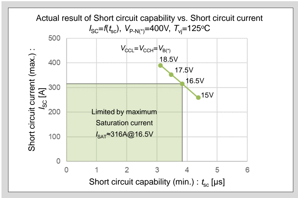
Fig.5 6MBP35XSJ(K)065-50 Short circuit capability and SCSOA
