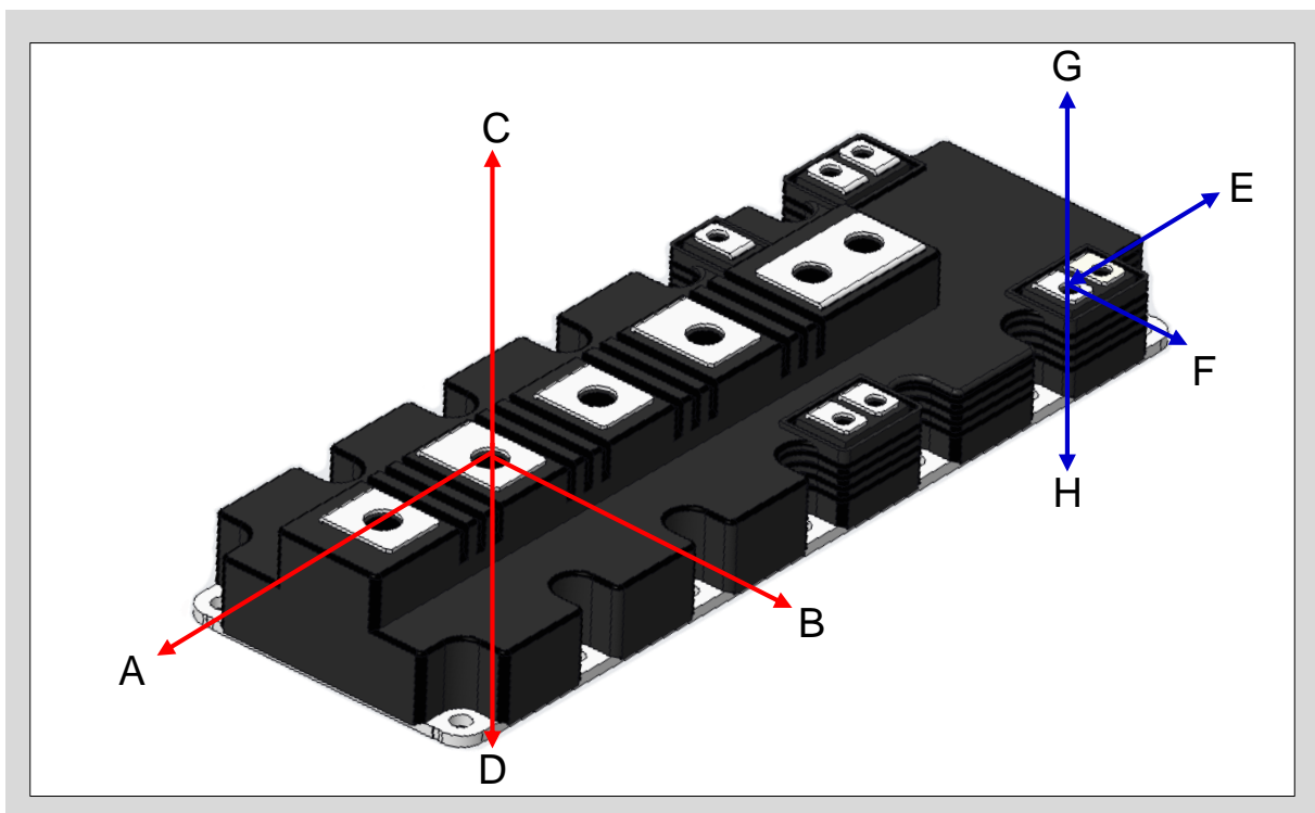
Fig.4 Allowable strength and application direction
