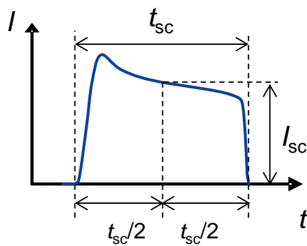
Short circuit current waveform
