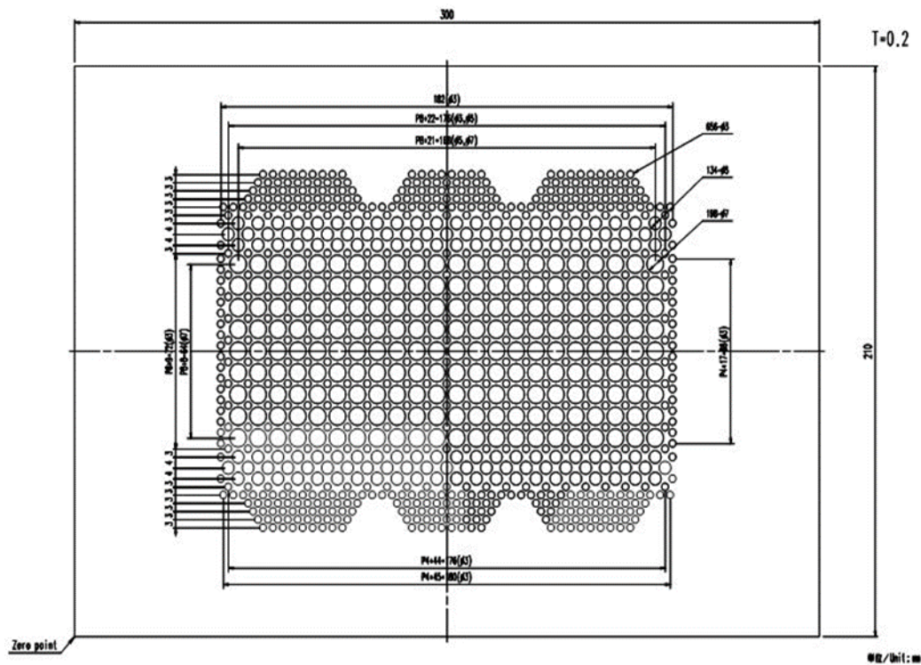
Figure 3. The example of the stencil mask for M152/M156 packages
