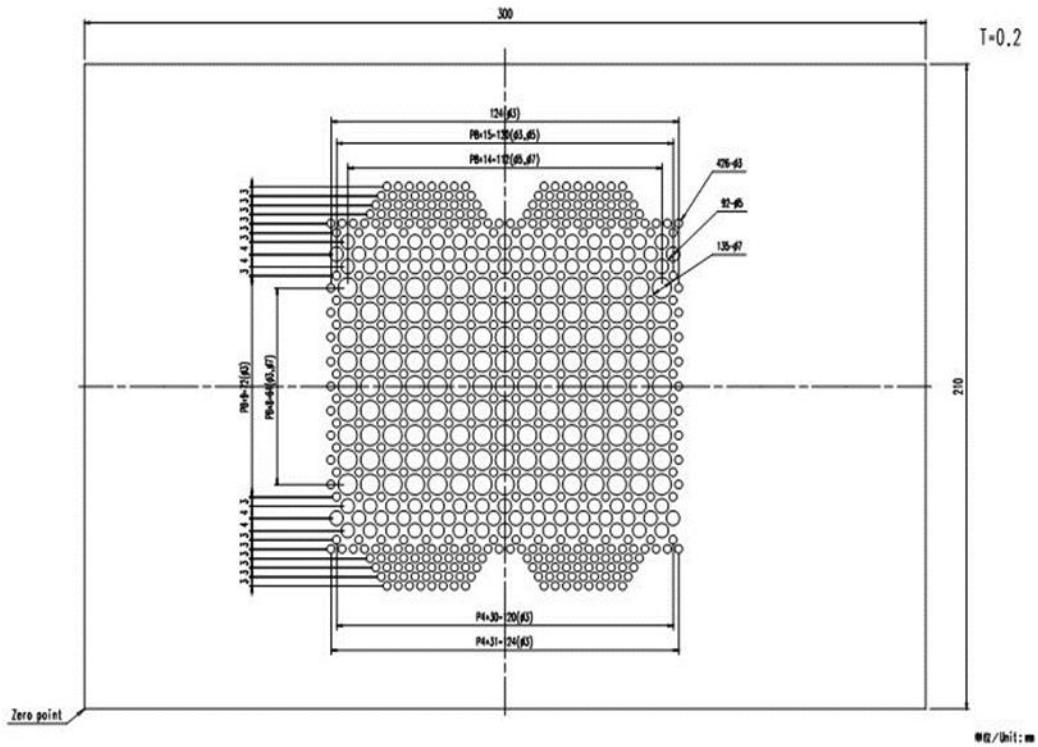
Figure 2. The example of the stencil mask for M151/M155/M256/M278 packages
