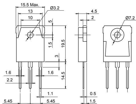
TO-3P
