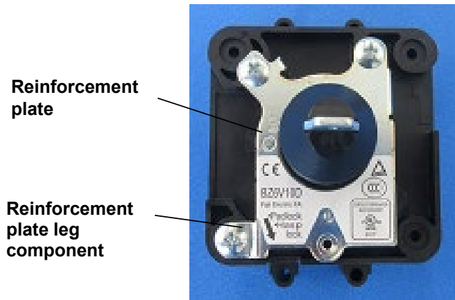
Driver unit
