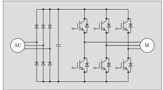
Figure Switching circuit
