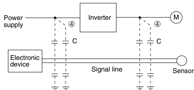
Fig. 5 Electrostatic noise
