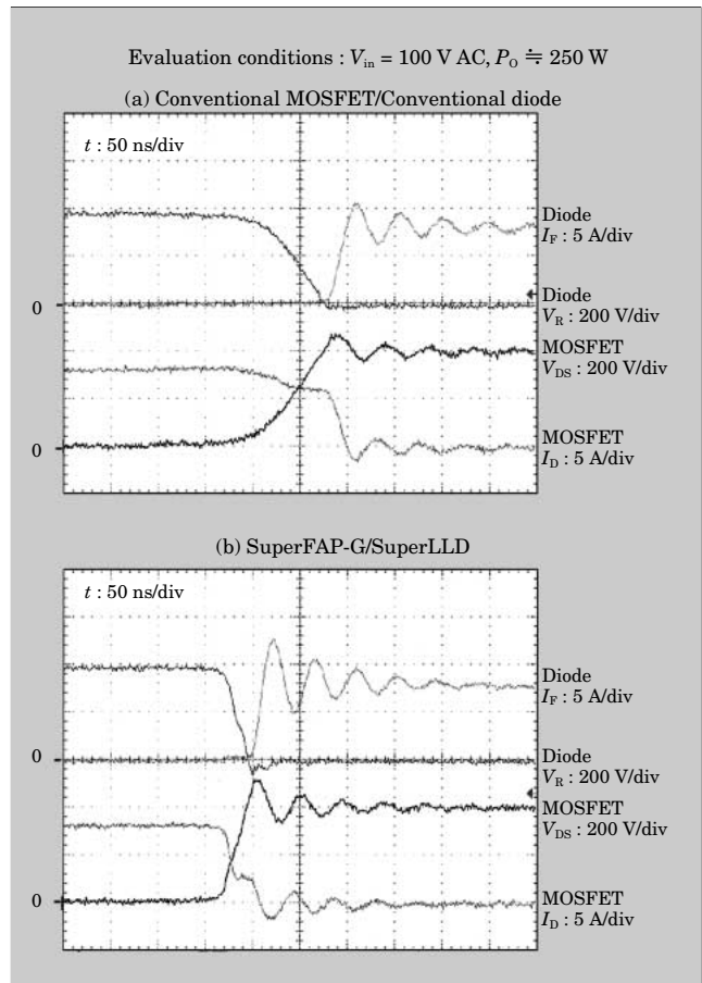
Fig.7 Continuous current mode PFC circuit (turn-off waveform)
