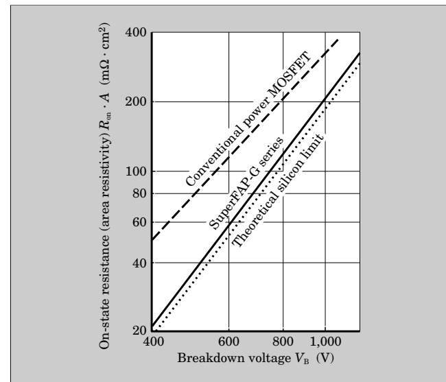
Fig.3 Relation between V_b and R_{on} \cdot A
