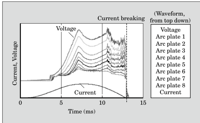
Fig.4 Example of arc plate measurement
