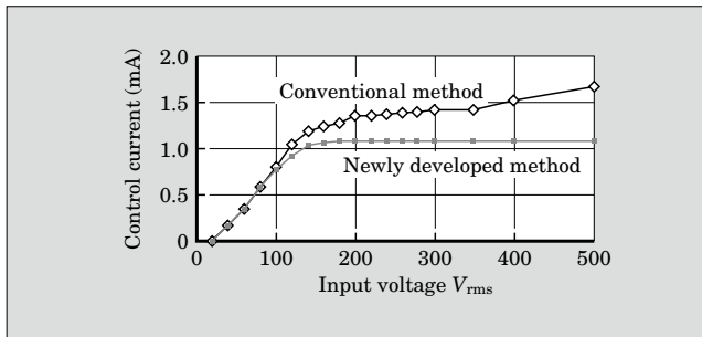
Fig.9 Comparison of power circuit characteristics
