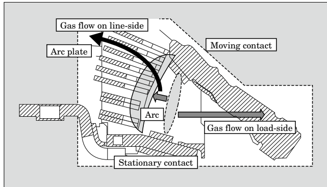
Fig.3 Schematic of current breaking operation
