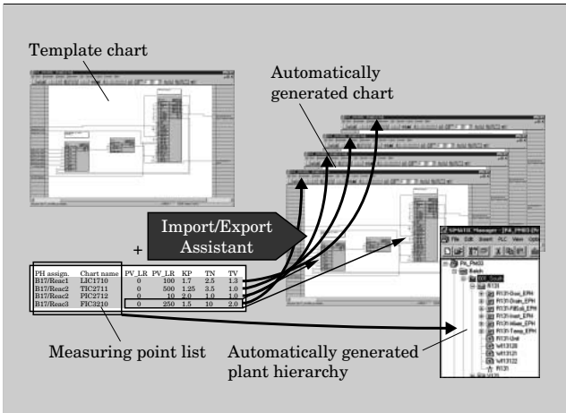
Fig.7 Import/export assistant
