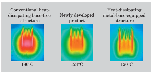
Fig.8 Thermo-photographs (at steady-state condition)
