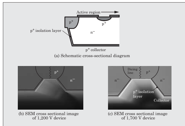
Fig.3 RB-IGBT structure and cross sectional images
