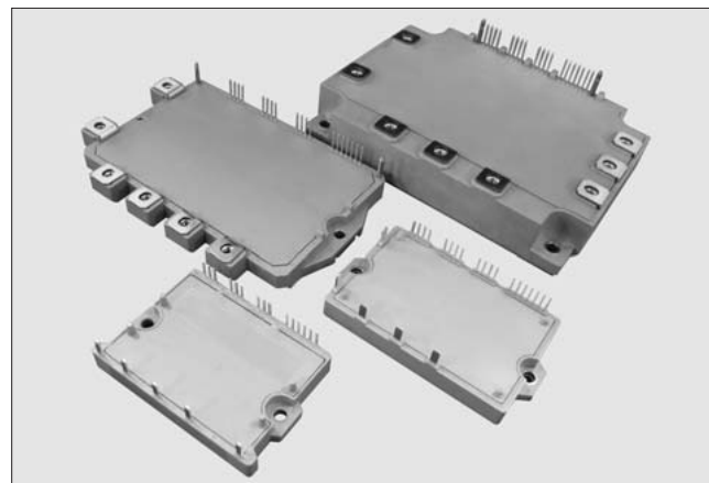
Fig.2 “V-Series” IPMs
