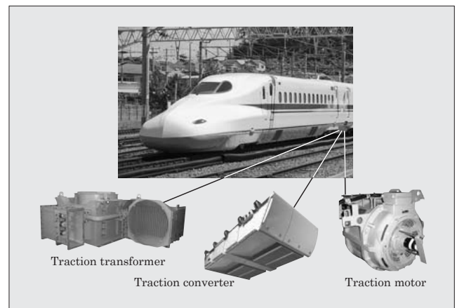
Fig.29 Electrical equipment for the N700A Shinkansen
