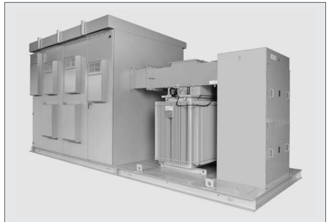
Fig.22 “PVI1000-3/1000”
