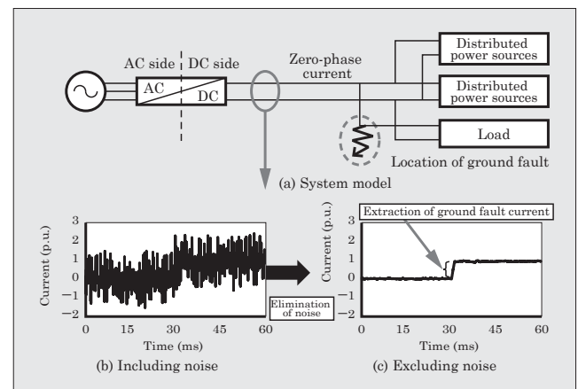
Fig.48 Grand fault analysis results
