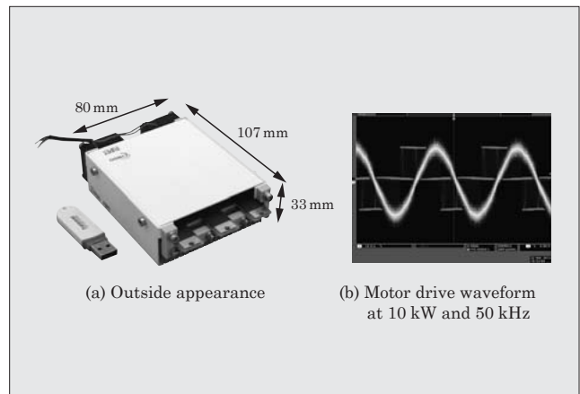
Fig.14 All-SiC inverter
